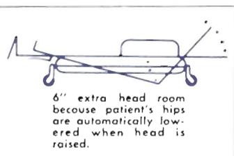
A-205 Heart Patient Cot Sketch shows design which affords extra head room.
